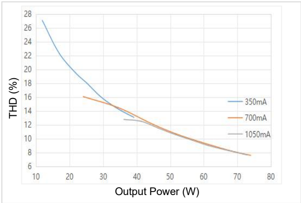
THD Curve
