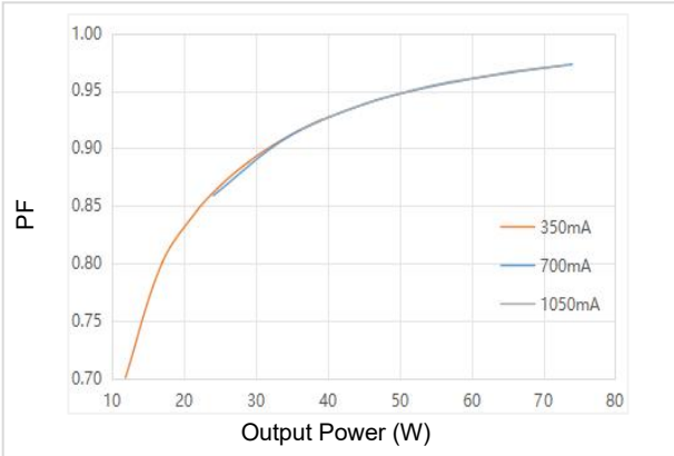
PF Curve
