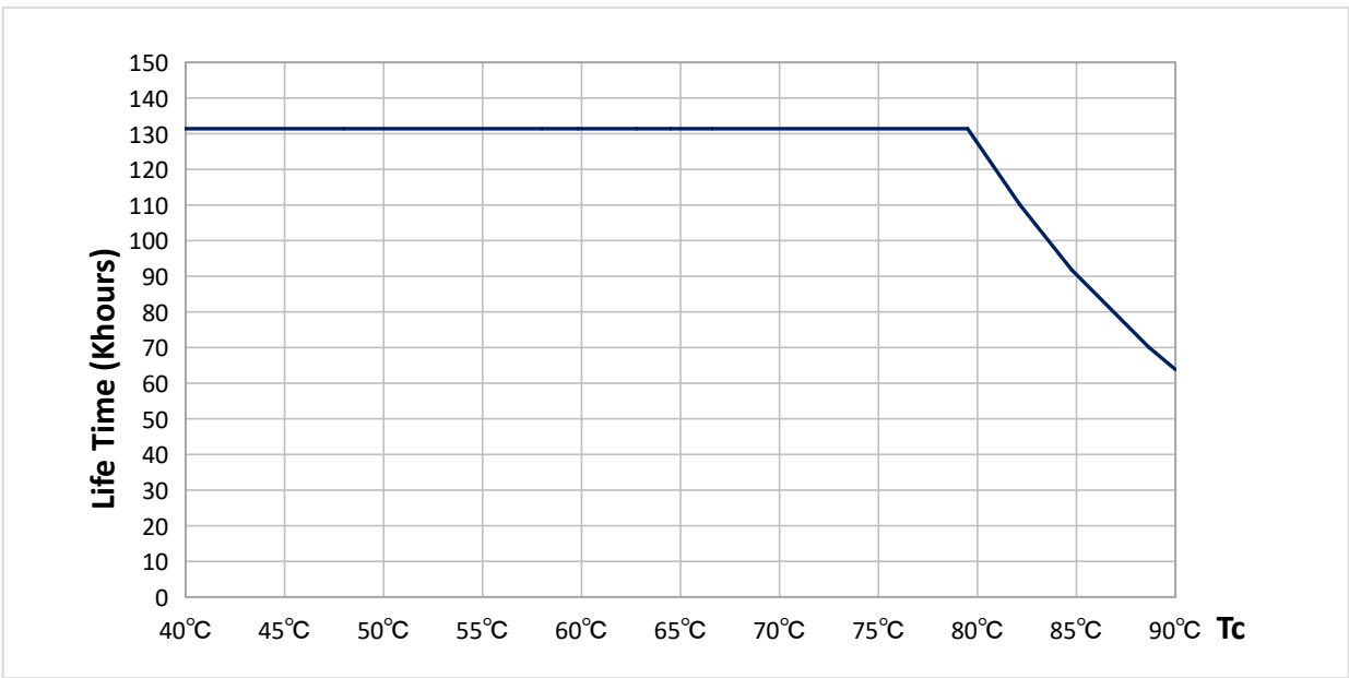
Lifetime Curve
